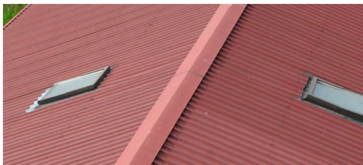
Pannelli sandwich Isometal (5G - in alto - SUPERCOPPO in basso) Isometal's sandwich panes (5G - above - SUPERCOPPO below)
